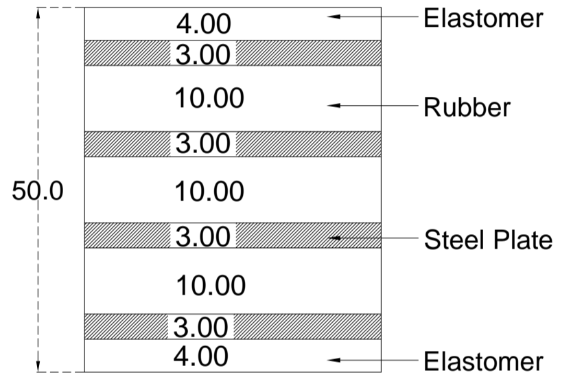
SECTION X-X
